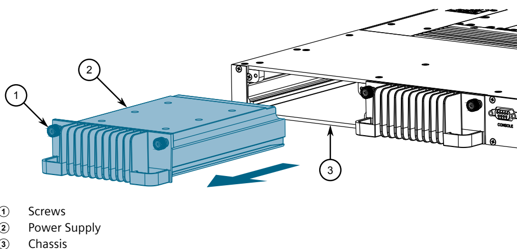
Figure 4.5 Removing a Power Supply
