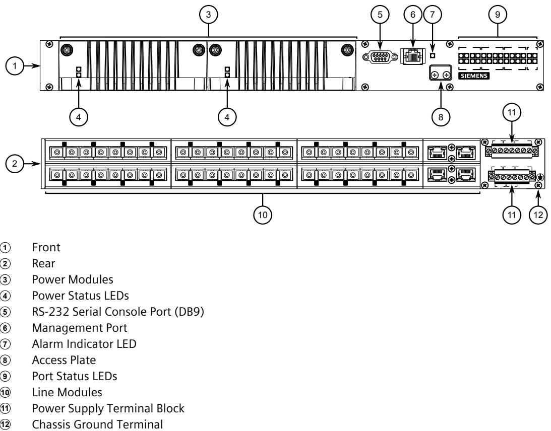
Figure 1.1 RUGGEDCOM RSG2488
