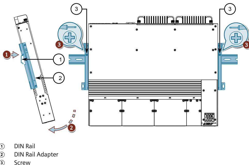
Figure 2.2 Mounting the Device to a DIN Rail
