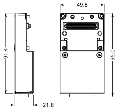
Figure 5.5 2-Port Line Module Dimensions
