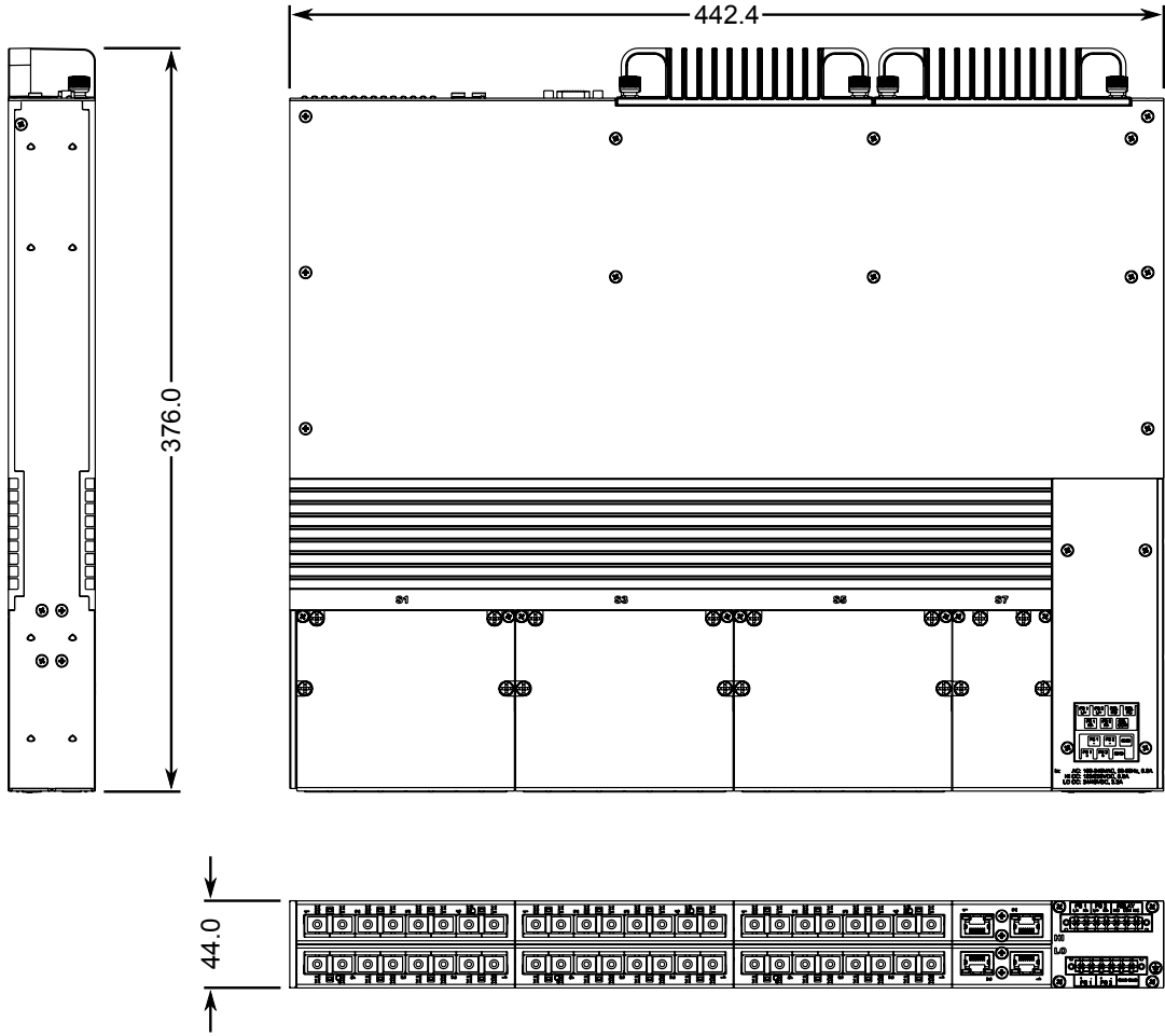
Figure 5.1 Overall Dimensions
